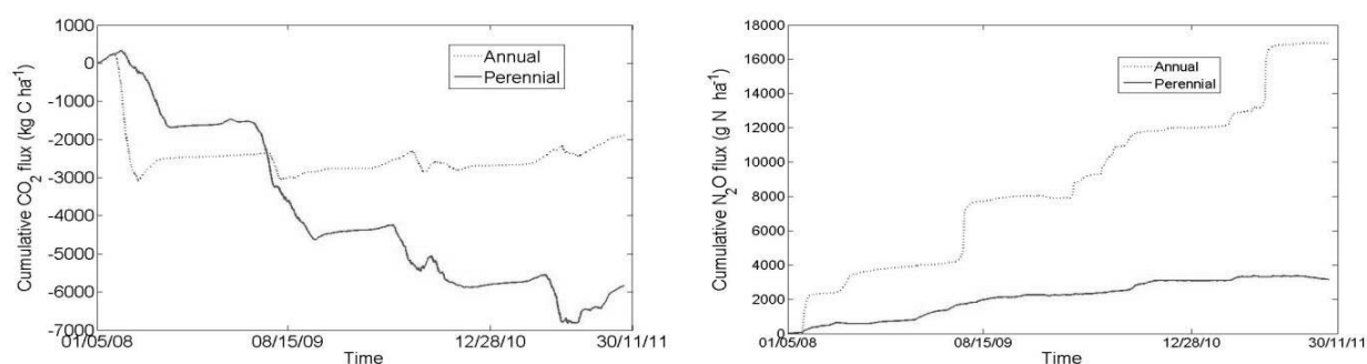
Figure 1: Cumulative C uptake (left) and N 2 O emission (right) by annual and perennial cropping system from 2008 to 2011. Positive numbers indicate a loss from the ecosystem to the atmosphere.
